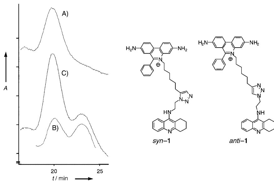
Figure 1. Left: HPLC analysis of thermal and AChE-templated assembly of TZZ and PA6 . A) Product from in situ assembly in the presence of AChE. B) Triazole 1 prepared by thermal reaction; equal amounts of syn and anti isomers were isolated. C) Solution (A) plus a small amount of solution (B). Right: syn - and anti -isomers of 1 .
